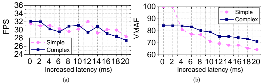
Fig. 19. Changes of FPS (a) and VMAF (a) as the server processing latency increases for each frame.
