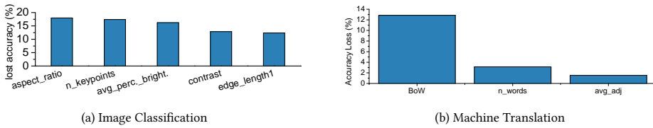
Fig. 9. The loss in accuracy when final chosen features are not used in our premodel. For image classification (a) we only show the top five. For machine translation (b) we show all 3.
