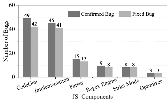
Figure 7. #COMFORT-found bugs per compiler component. defineProperty API. All versions of V8 tested fail to correctly compile the test case shown in Listing 1. This test case contains a “type error” because the length property at line 3 is not configurable but the code tries to change it. Such an attempt should lead to a TypeError exception, but V8 allows the code to be successfully compiled. This bug is exposed by generating a test data to manipulate a non-configurable property of the array object according to ECMA-262. We were the first to report this bug. This test case also exposes a bug of Graaljs for the same reason.
