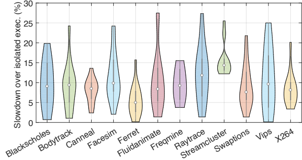
Figure 15. The slowdown distribution of computation-intensive PARSEC benchmarks when they run with a Spark task under our scheme. The baseline is running the target application in isolation.
