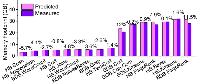
Figure 17. Predicted memory footprints vs measured values for HiBench (HB) and BigDataBench (BDB).
