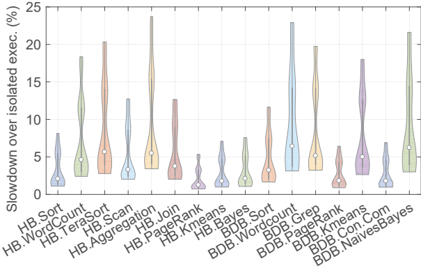
Figure 14. Violin plot showing the distribution of slowdown when using our scheme to co-locate the target benchmark with another application on a single host. The baseline is running the target application in isolation. Here we run each of the 16 target benchmarks from HiBench and BigDataBench along with each of the remaining 43 benchmarks.
