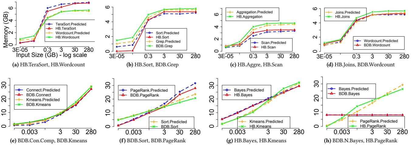
Figure 18. Comparisons of the predicted memory footprint to the measured value. This set of memory functions can precisely capture the memory requirement of our benchmarks.
