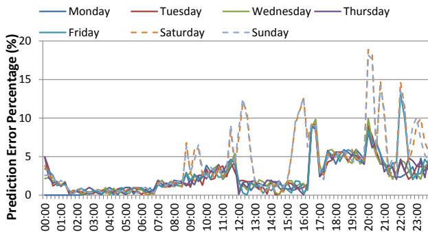
Figure 4: Prediction error percentage per day.
