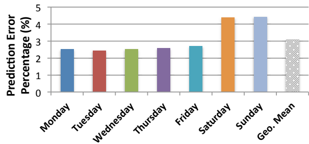
Figure 5: Average prediction error percentage per day.
